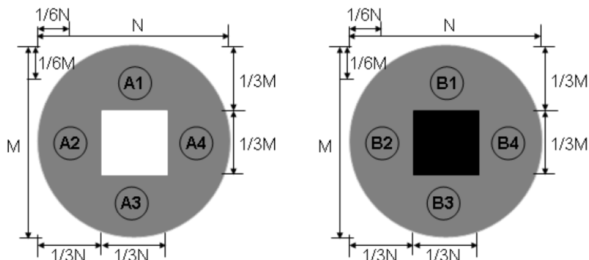
Cross-talk Test Pattern
