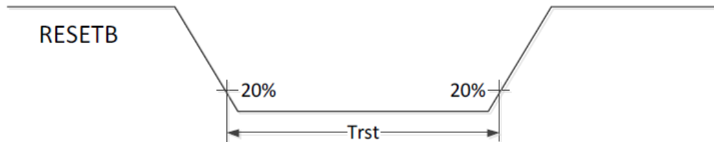
Figure: Reset timing
