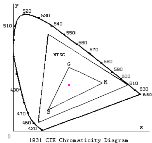
Fig. 1931 CIE chromaticity diagram
