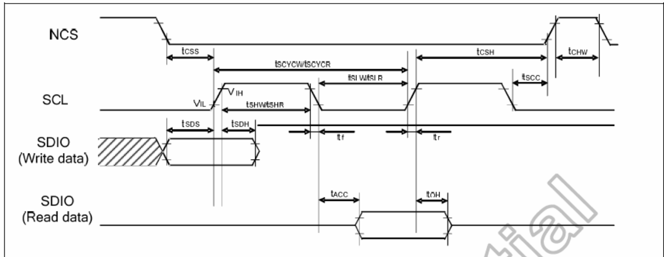
Figure 8-4: Serial interface characteristics
